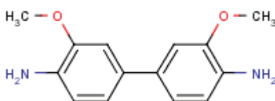
Figure 1. 3,3'-Dimethoxybenzidine Structure
