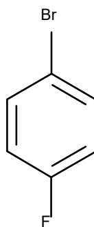
Figure 1. 1-Bromo-4-fluorobenzene Structure
